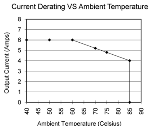
Figure 3.0: Current Derating
