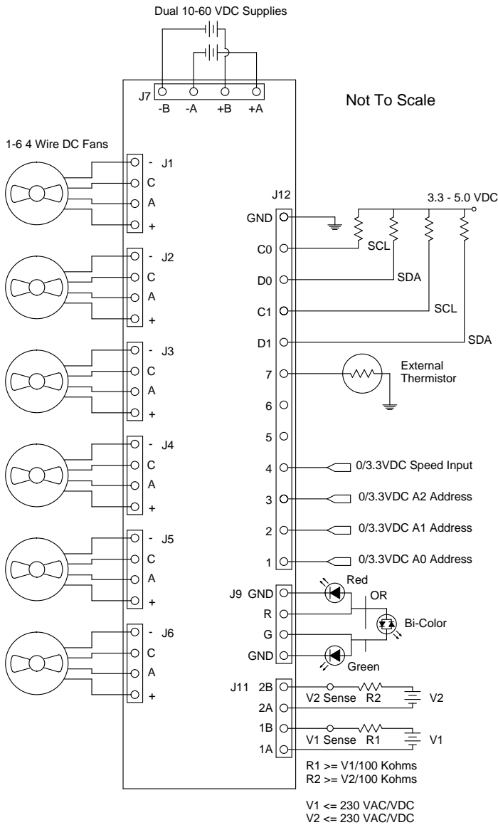
Figure 2.0: Connection diagram showing input power, fan, interface, temperature sensor, LEDs and alarm connections for a Cirrus-6 Fan Control.
